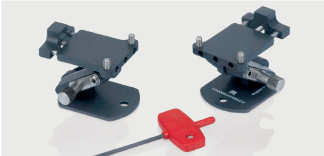
Technical data Dimension: 67 x 35 x 46 mm Weight: 157 g
