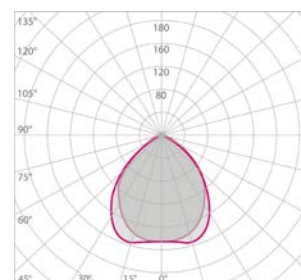
Curva fotometrica Photometric diagram
